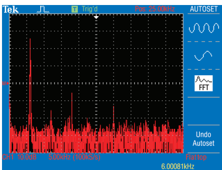
Fast Fourier Transform (FFT) makes it easy to precisely analyze, characterize and troubleshoot circuits in the frequency domain.
